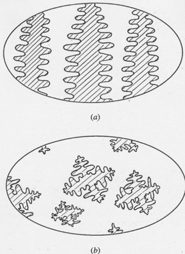
Fig. 1—Schematic illustration of the averaging volume containing (a) columnar dendritic crystals and (b) equiaxed dendritic crystals.
